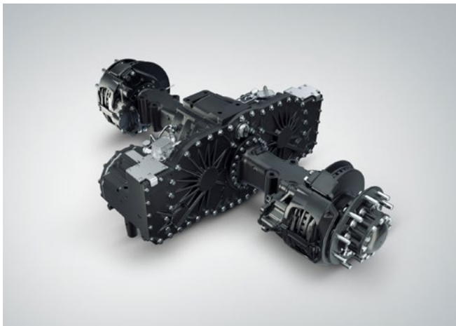
eAxle
